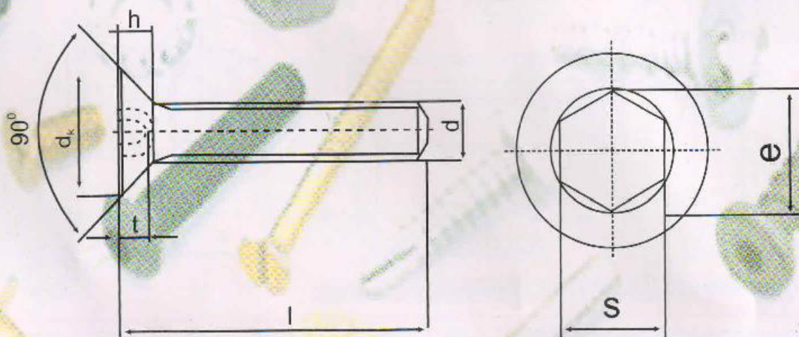
Hexagon Socket Countersunk Head Screws
